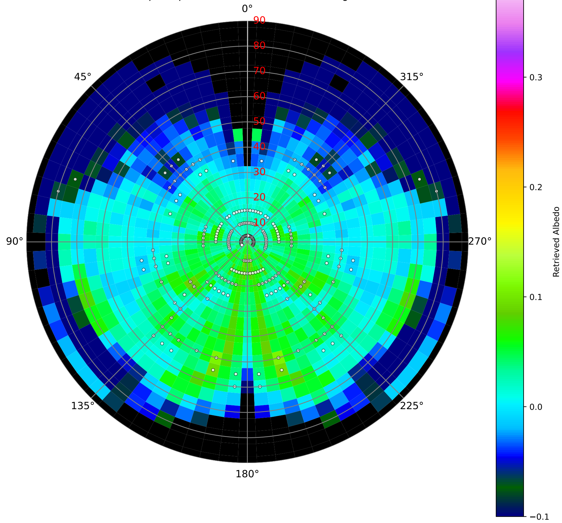
1.27 \mu\text{m} Equatorial Dunes. Incidence: 55 degrees
